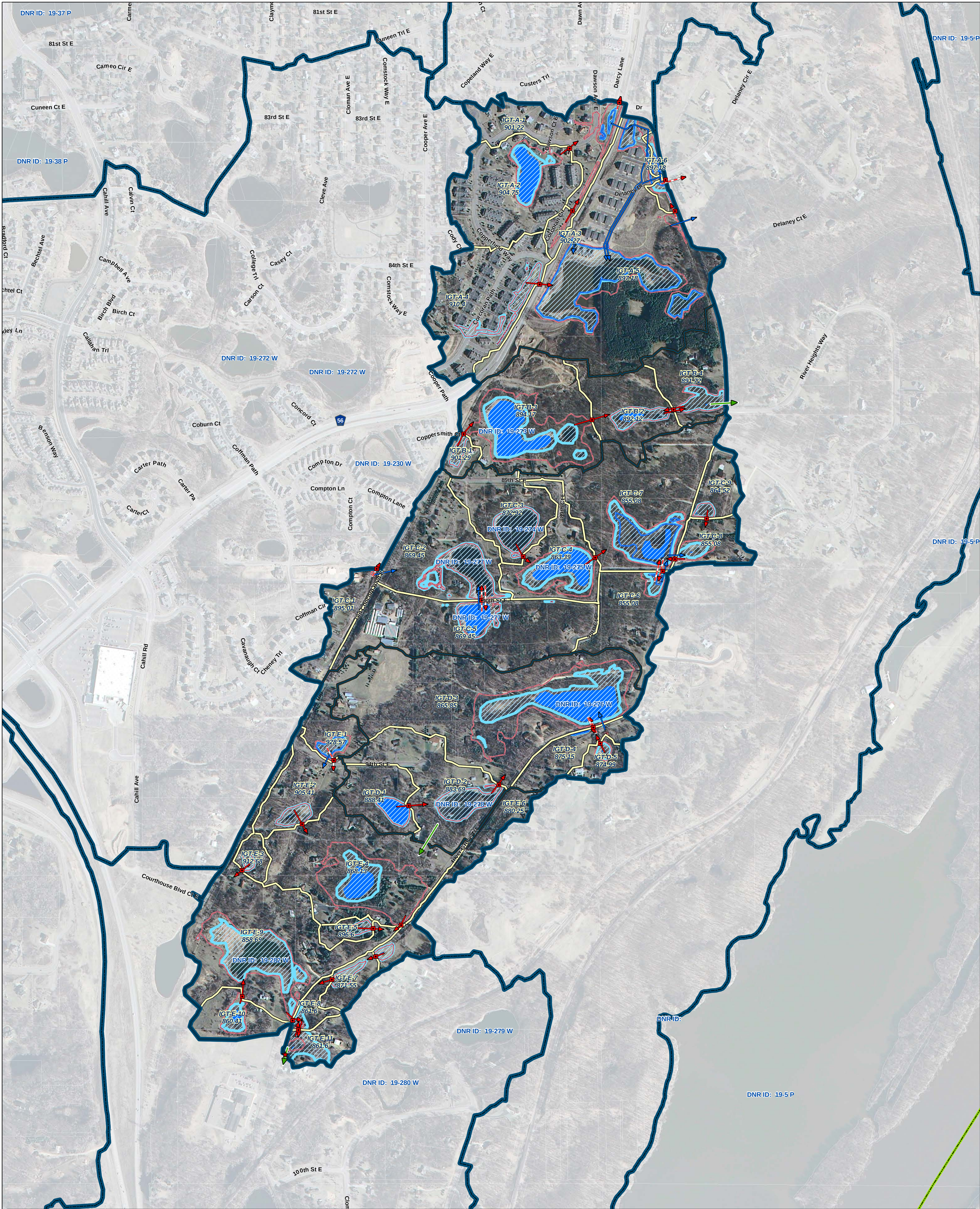
Figure 2-19A INVER GROVE TRAIL DRAINAGE BASIN 100 Year Snowmelt Modeling Results Inver Grove Heights Water Resources Management Plan
