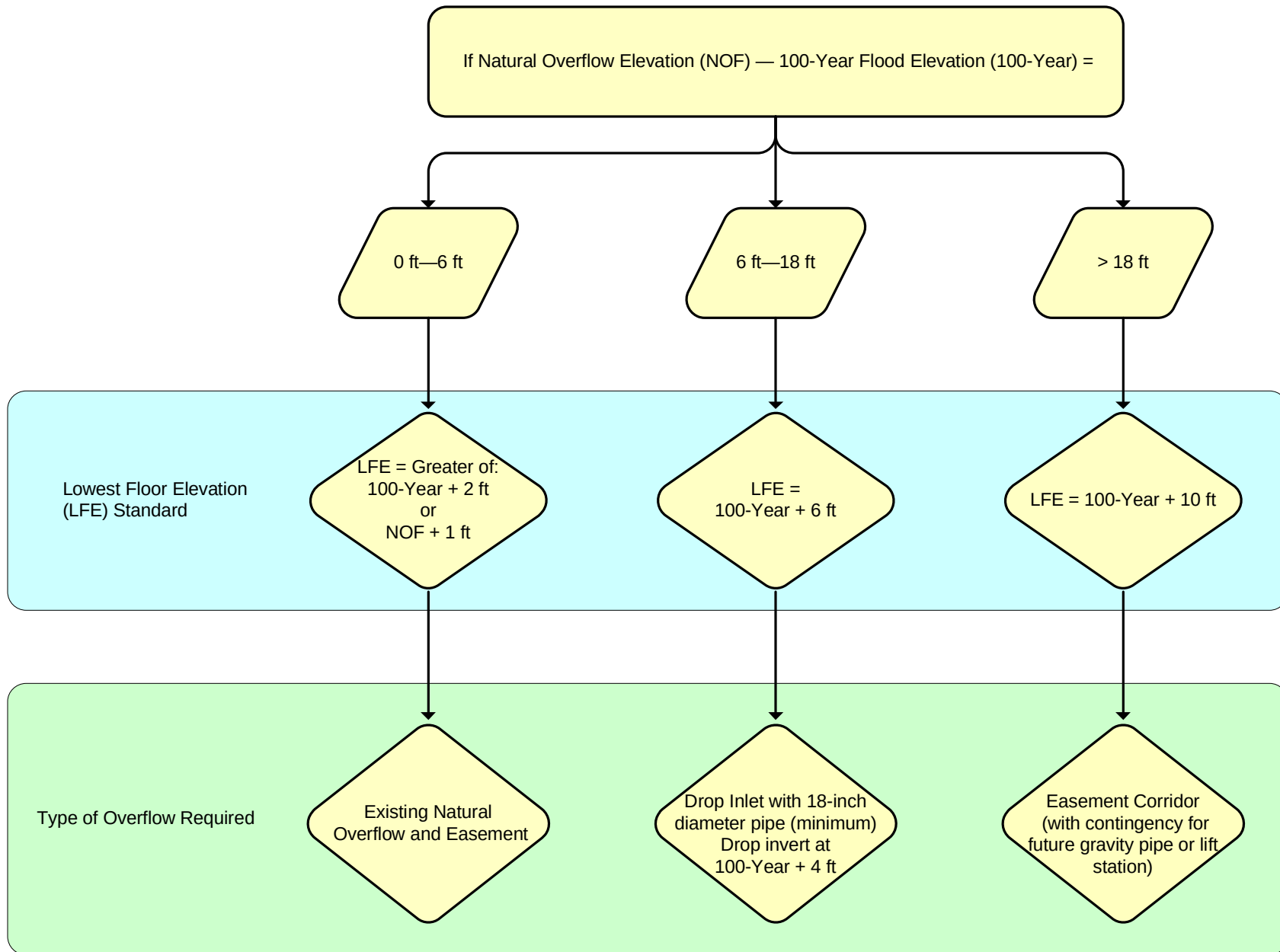
Figure 3-1 LOWEST FLOOR ELEVATION STANDARDS AND TYPE OF OVERFLOW—LANDLOCKED BASINS Inver Grove Heights Water Resources Management Plan
